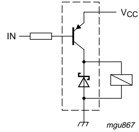
Fig 9. Inductive load driver (relays, motors and buzzers) with free-wheeling diode.
