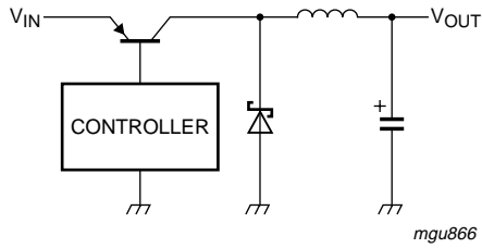
Fig 8. DC-to-DC converter.
